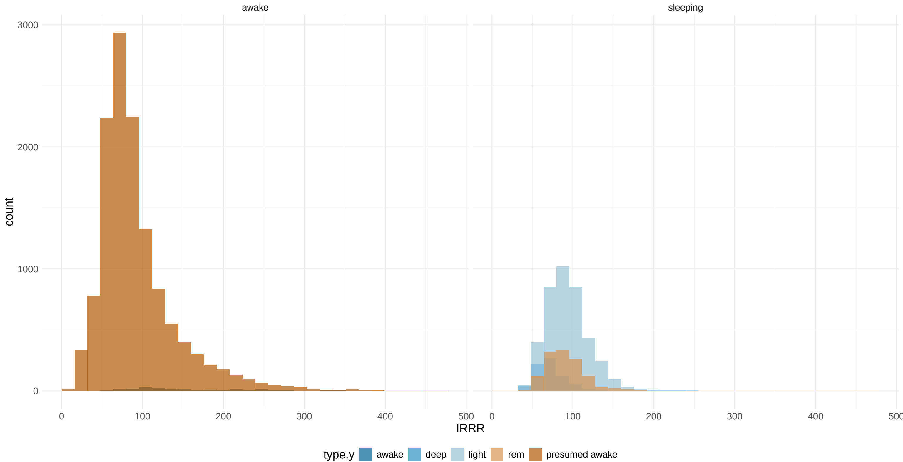
Histogram of IRRR for FLARE005 split by waking and sleeping stages Colour indicates sleep pattern
